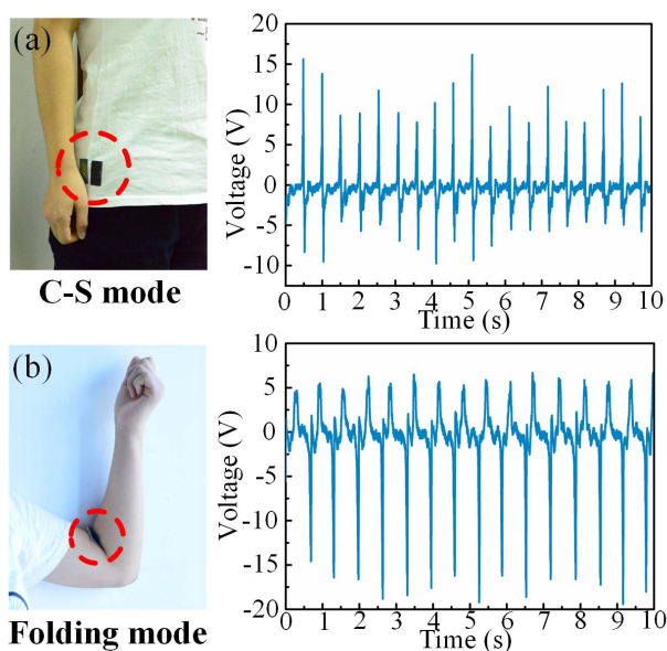
Figure 8: The optical images and corresponding output voltages when the thin-film generator was fixed at different positions of human body.
