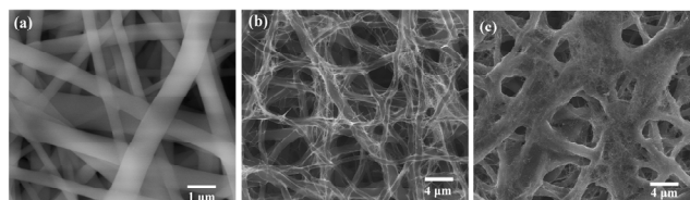
Figure 3: SEM images of the (a) PU nanofibers, (b) fibers coated with AgNWs, (c) fibers coated with AgNWs & CNT.
